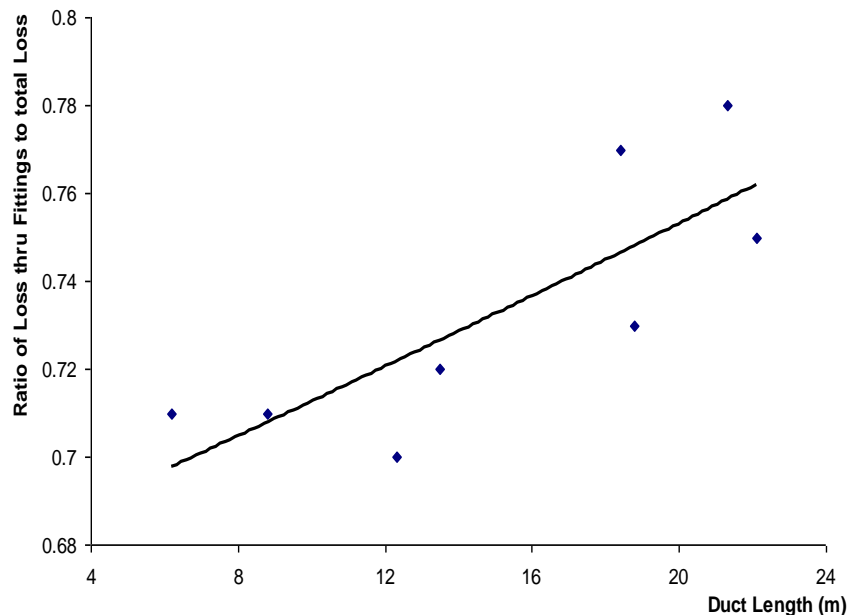
Figure 2: Variation of Fitting Loss Fraction with Duct Length
